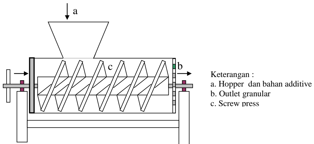
Gambar 1. Mesin Granulator Tipe Screw
